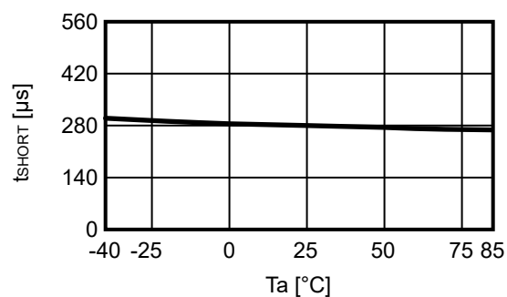
3.8 t_{SHORT} - T_a
