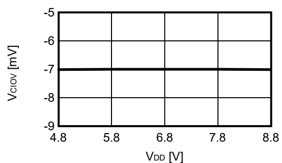
2. 11 V_{\text{CI OV}} - V_{\text{DD}}
