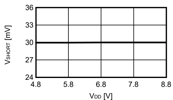
2. 9 V_{\text{SHORT}} - V_{\text{DD}}
